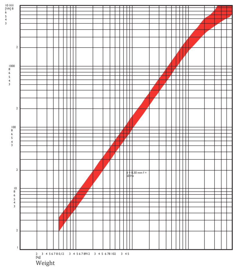
Appearant power of single phase core
