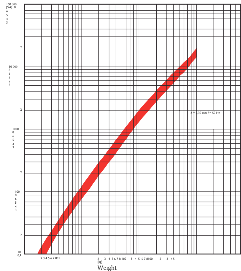
Appearant power of three phase core
